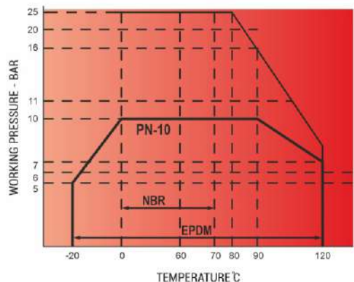
PRESSURE/TEMPERATURE DIAGRAM
