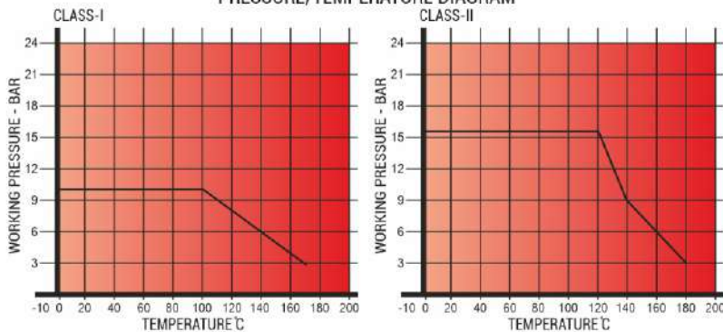
PRESSURE/TEMPERATURE DIAGRAM
